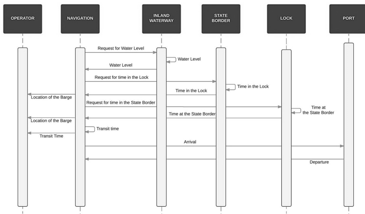
Fig. 4. Agents' communication at Navigation
