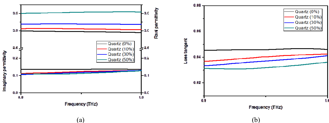
Figure 1: (a) measured permittivity. (b) measured loss tangent.
