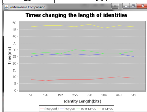
Figure 3: Times changing the length of identities
