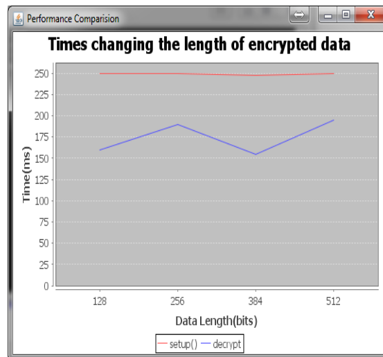
Figure 6: Times changing the length of encrypted data
