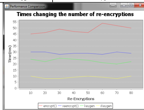
Figure 2: Times changing the number of re-encryptions
