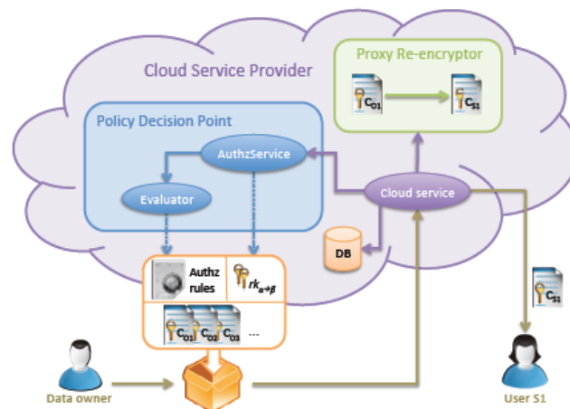
Figure 1: Architecture of System Model
