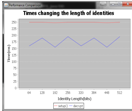
Figure 4: Times changing the length of identities
