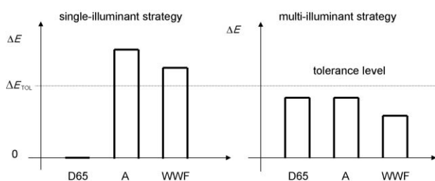
Figure 1. Possible predicted colour differences \Delta E_{D65}, \Delta E_A, \Delta E_{WWF} of two recipes (against the given standard) using the same combination of colorants. The strategy \Delta E_{D65} \rightarrow 0 was used on the left, and the strategy \max\{\Delta E_{D65}, \Delta E_A, \Delta E_{WWF}\} \rightarrow 0 on the right.
