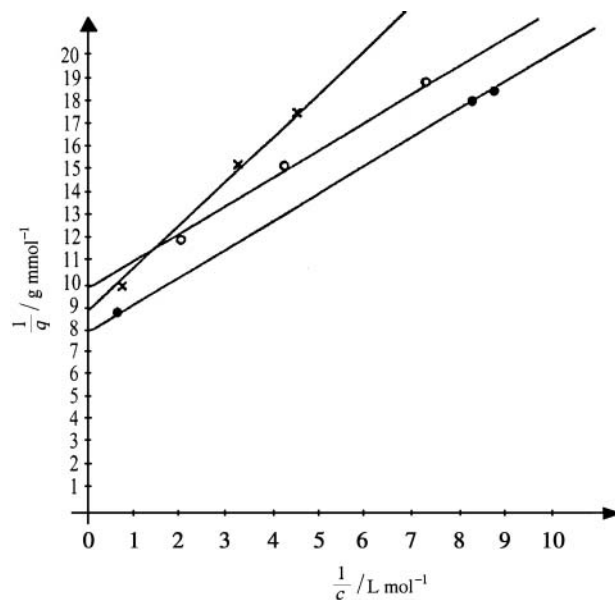
Figure 4. Linear Langmuir plots of Ag I (●), Cd II (○), Pb II (×) cations retention on hemp-SH.
