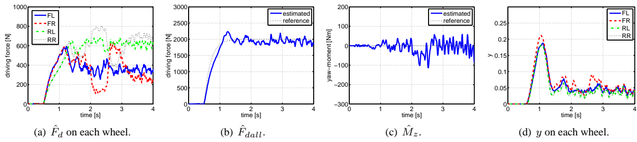
Fig. 20. Experiment of split slippery road (only DFC).
