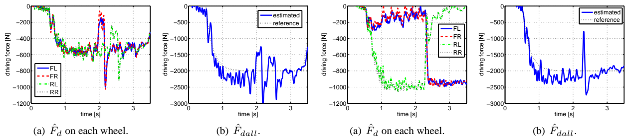
Fig. 22. Deceleration test (only DFC).
