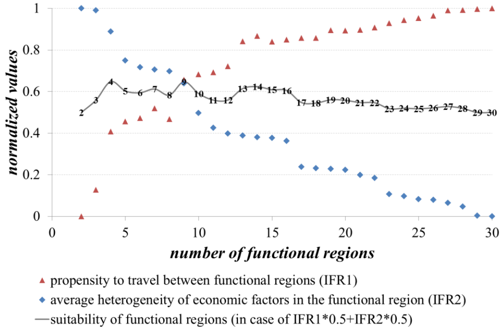
Figure 1: Suitability of functional regions (more stable regions are in local maximums) modelled by Intramax method and equally weighted criteria in Slovenia in 2010.
