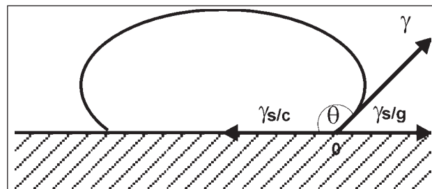
Figure 1 Equilibrium at the solid-liquid-gas interface
