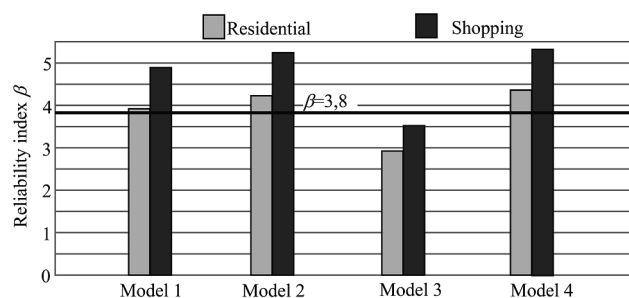
Figure 5 Reliability indices for different construction purposes
