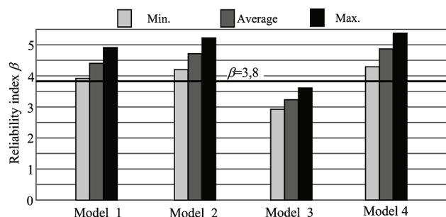
Figure 4 Reliability indices for different calculation resistance models
