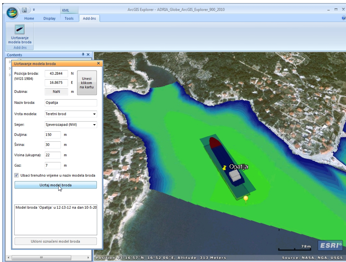
Figure 5: 3D model simulation of ship entering chosen place of refuge.
