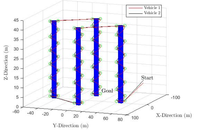
Fig. 13: Smaller platform with tighter inspection - 3D view
