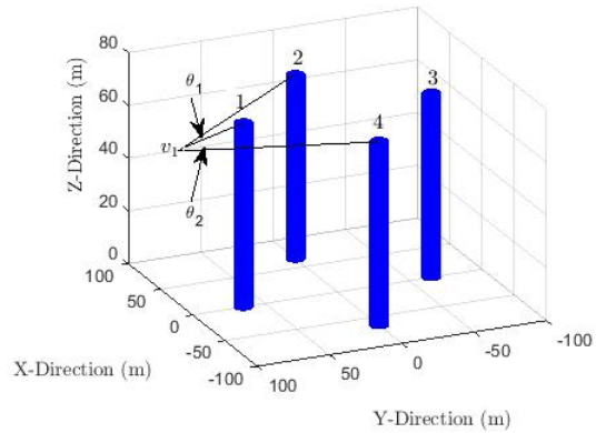
Fig. 6: Initial distance and angle calculations
