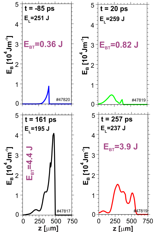
FIG. 7. The integrated energy in the SMF as a function of the distance z from the target calculated using Eq. (3) for selected times.
