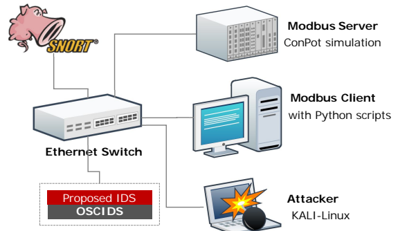
Figure 5: Experimental Test-bed Architecture
