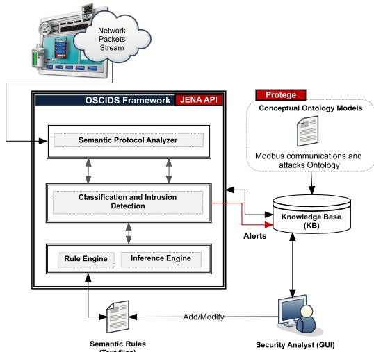
Figure 2: Overall OSCIDS Framework Architecture
