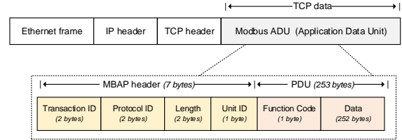
Figure 1: Modbus TCP packet structure
