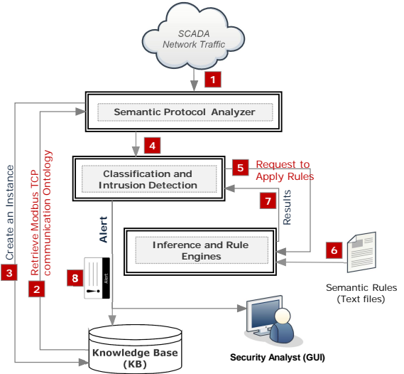
Figure 3: OSCIDS Framework Work-flow
