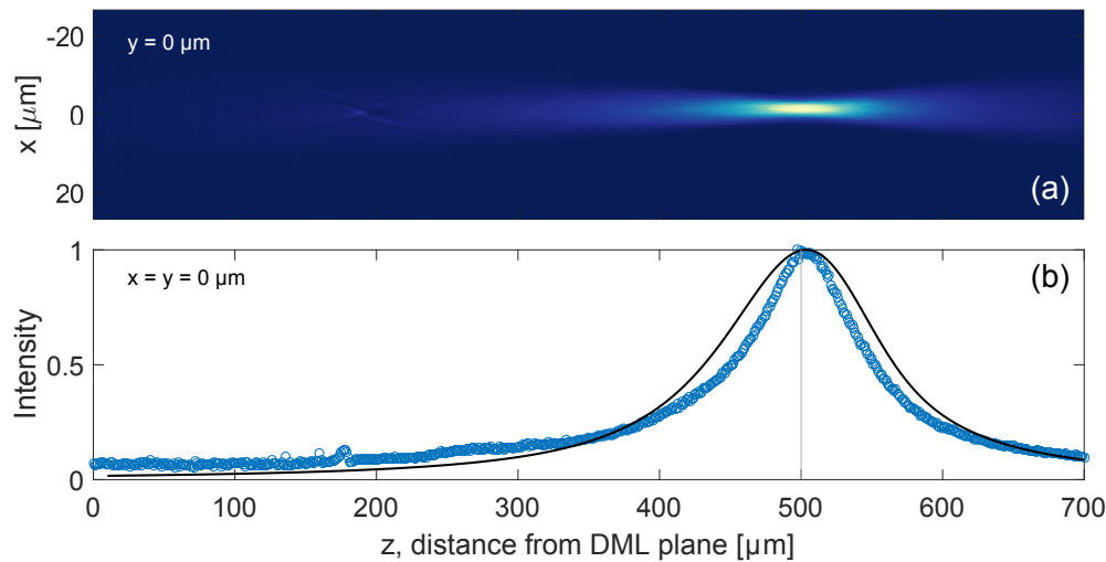
Fig. 6. Measured propagation of lens 2, designed to focus at 500\ \mu\text{m} . (a) Color map of the measured beam profile after the DML plane. Dark represents an intensity of 0, and bright represents a normalized intensity of 1. (b) The measured intensity (open circles) along the optical axis, z , with equivalent simulation of the design profile for comparison (solid line).
