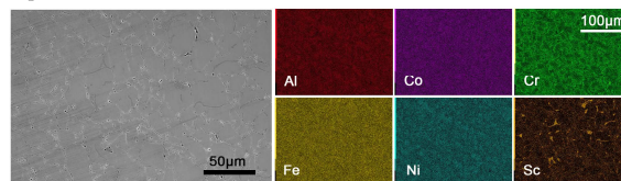
j Al 2 CoCrFeNi+Sc sintered powder - 9.5 GPa, 1500 K, 30'
