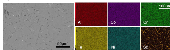
h Al 2 CoCrFeNi+Sc sintered powder - 9.5 GPa, 1000 K, 30'
