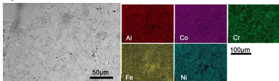
i Al 2 CoCrFeNi sintered powder - 9.5 GPa, 1500 K, 30'
