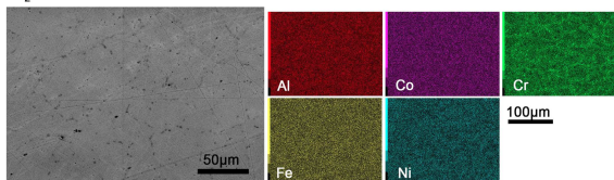
e Al 2 CoCrFeNi sintered powder (SPS) - 0.05 GPa, 1123 K
