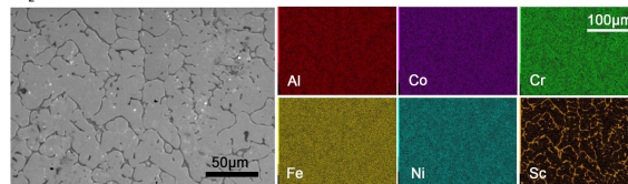
f Al 2 CoCrFeNi+Sc sintered powder - 2.1 GPa, 1253 K, 1h
