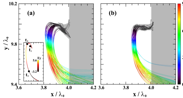
Fig. 6. Typical trajectories of representative electrons from the incline surface of a blazed grating (a) and a normal grating (b) targets with only single protuberance. The temporal duration of the trajectories is from t = 4.2 T_0 to t = 6.4 T_0 . The color bar of trajectories represents the electrons energy \gamma . The inset in (a) shows the acceleration and radiation period of a single grating target electron, the color bar represents the transverse electric fields felt by the electron, which is normalized by mc\omega_0/e . The gray regions show the initial profiles of the two targets.
