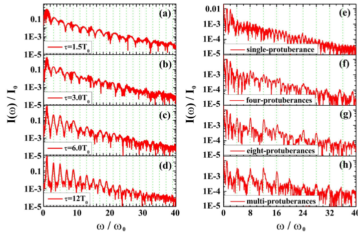
Fig. 5. The radiation spectra collected at reflected direction from a plane target interaction with lasers of different cycle numbers (a)-(d). The radiation spectra collected at 7.6^\circ from grating targets with different protuberance numbers (e)-(h).
