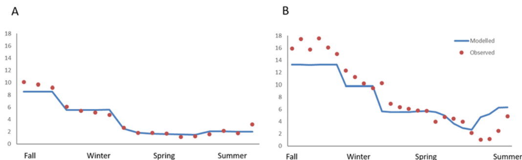
Fig. 7. SiO 2 model fit (daily) across two sub-catchments of Simcoe with contrasting soil types; A) Ramara (60% clay; R 2 0.97) and B) Orillia (6% Clay; R 2 0.87).
