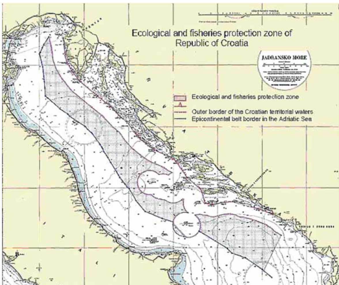
Fig. 1. Environmental and Fisheries Zone of the Republic of Croatia (BAJIĆ & TOMAŽIĆ, 2007)
