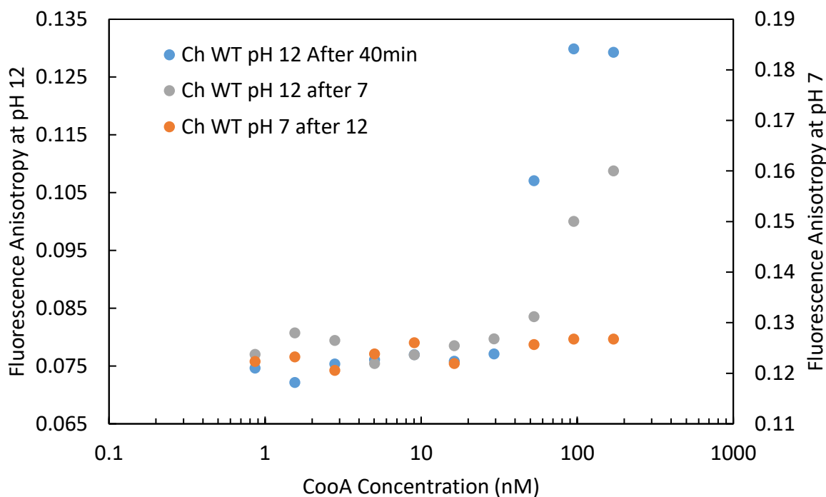
Figure 8. Fluorescence anisotropy reversibility experiment of Ch CooA samples with Texas Red DNA taken at pH 12 then 7 and 12 to demonstrate reversibility. pH 7 provides a stable flat line, indicating no binding, while binding returns in the pH 12 sample. The secondary pH 12 curve shifts slightly to the right due to moderate protein denaturation over time.
