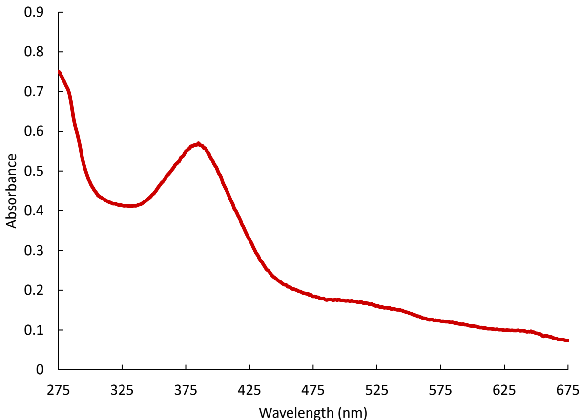
Figure 11. Electronic absorption spectrum of D72A CoxA at pH 3. 75mM phosphate pH 3 buffer with 100mM sodium chloride was used as a blank. The Soret peak is at 387nm, consistent with a 5-coordinate, high-spin heme.
