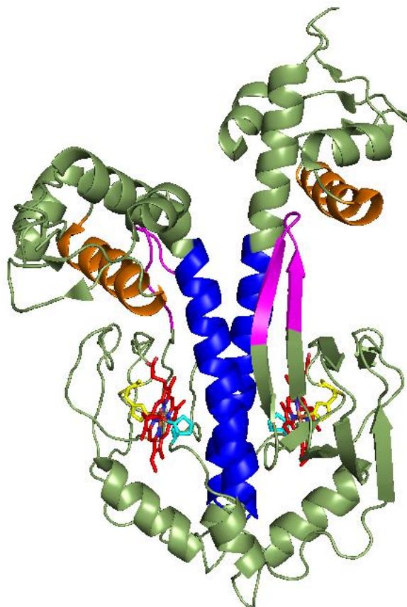
Figure 1. Inactive structure of CooA derived from Rhodospirillum rubrum (PDB 1FT9). 2 The b-type hemes are shown in red. The N-terminal heme ligands are shown in cyan. The distal heme ligands are shown in yellow. The conserved \beta 4/5 loops are shown in purple. The central C helices are shown in blue. The F helices that bind the major groove of DNA upon conformational change are shown in orange.
