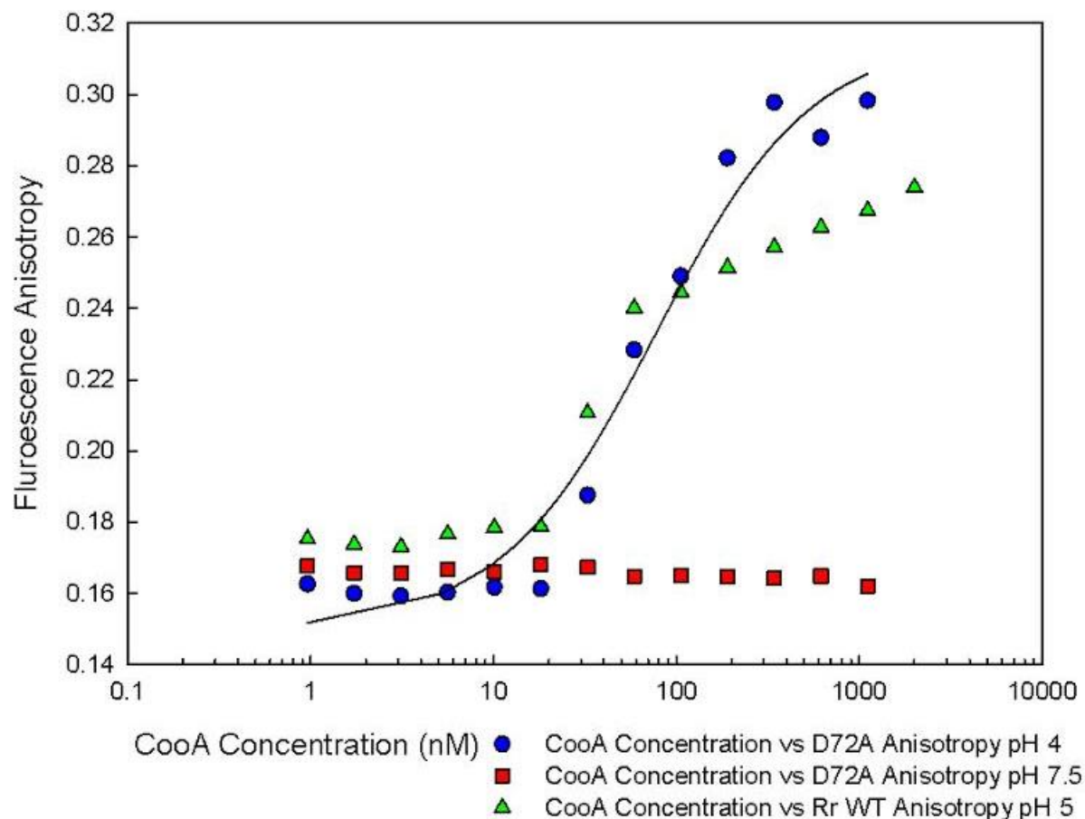
Figure 10. Fluorescence anisotropy curves of Rr. CooA variant, D72A, at pH 4 and 7.5. The Fluorescence anisotropy curve from Rr. Wt at pH 5 is included for comparison. At pH 7.5, no DNA binding is observed, while Wt -like activity of this variant is exhibited at pH 4.
