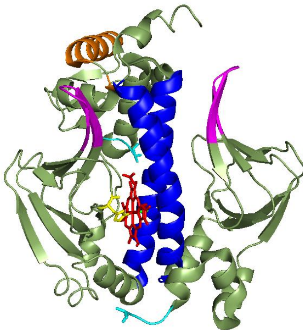
Figure 3. Active structure of CoxA derived from Carboxydothemus hydrogenoformans (PDB 2HKX). 7 The hemes are shown in red. The N-terminal heme ligands are shown in cyan. The distal heme ligands are shown in yellow. The proximal heme ligand, CO, is shown in green. The conserved \beta 4/5 loops are shown in purple. The central C helices are shown in blue. The F helices that bind the major groove of DNA are shown in orange.
