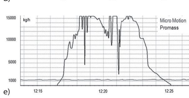
Fig. 10. Output values without slurry flowing
