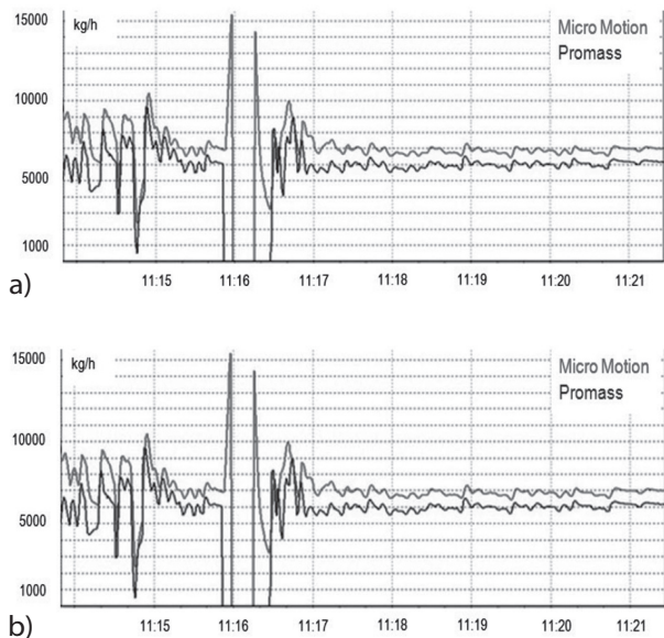
Fig.12. Transient state for product with \rho = 1.7
