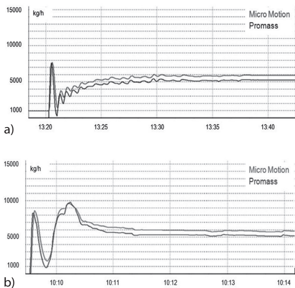
Fig.11. Transient state for product with \rho = 1.2
