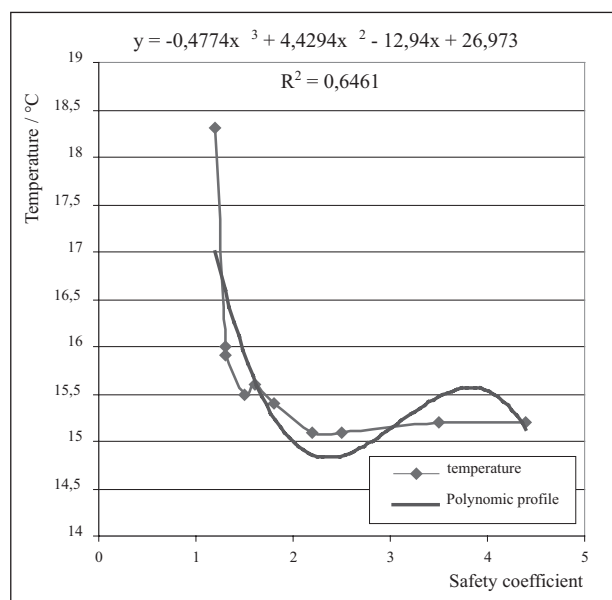
Figure 5 Relationship between temperature and safety coefficient in sample. Safety coefficient is on x axis, and measured temperature by thermographic method is on y axis.
