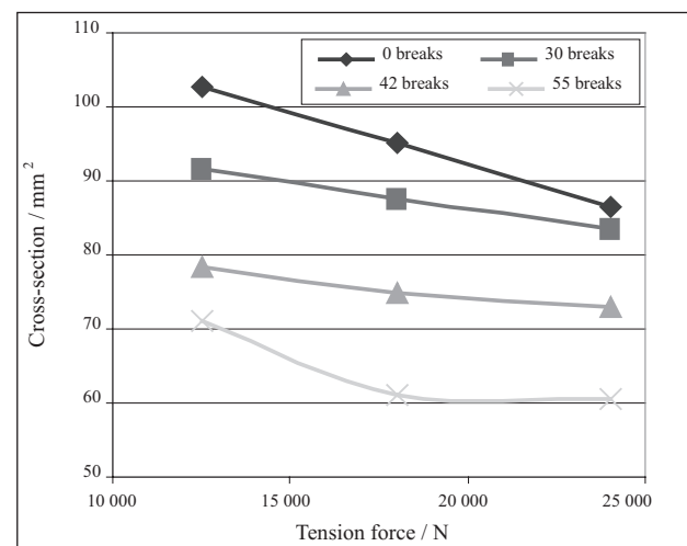
Figure 2 Dependence of the measured cross-section from the tension force in the unperturbed rope and ropes with various numbers of perturbed wires. Tension force F applied along the wire axis is on x axis, and cross-section obtained by acoustic method is on y axis. The value of cross-section was calculated from Eq. 4 with use of the measured values of parameters by acoustic method, the tension force F , mass density \rho , wire rope prolongation \Delta l_{\sigma} , and velocity of propagation of sound in the rope v .
