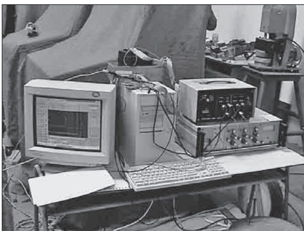
Figure 3 Acoustic method measurement set up. Acoustic analysis part of the set up.
