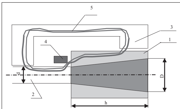
Figure 1 Rise of irrelevant indications within steel wire rope at the anchor. 1 is a conical cable end, 2 is a steel wire rope, 3 is a magnetic yoke, 4 is a point where irrelevant indication arises, 5 represents magnetic flux force lines.
