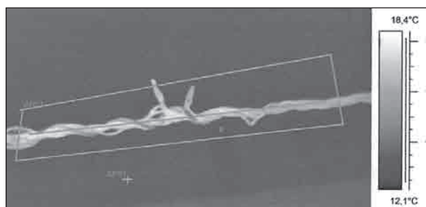
Figure 6 Ruptured steel wire rope. Thermogram – transformed infrared field into visible spectra.
