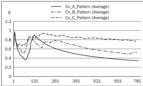
Figure 7 - Coefficient of Variation associated with retailer's orders
