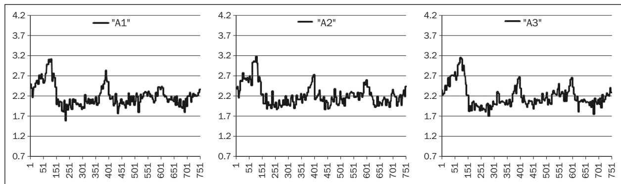
Figure 3 - Series disturbed by low variability
