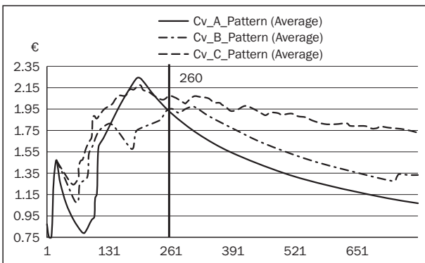
Figure 8 - Coefficient of Variation associated with wholesaler's orders
