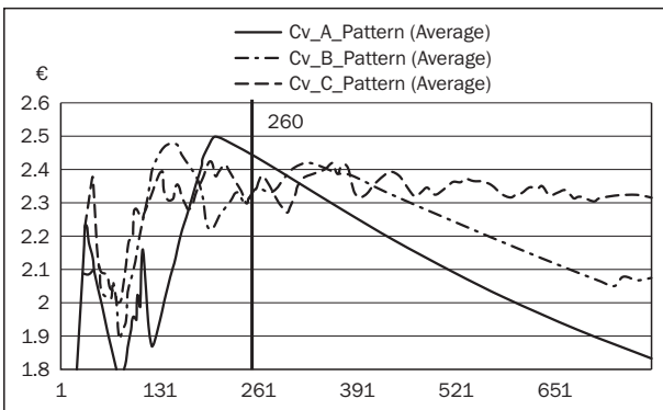
Figure 9 - Coefficient of Variation associated with manufacturing orders
