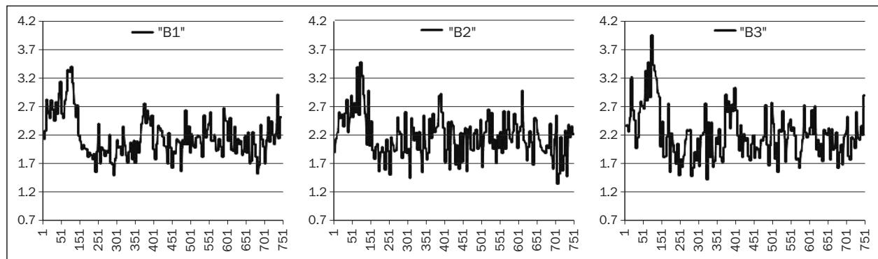
Figure 4 - Series disturbed by medium variability
