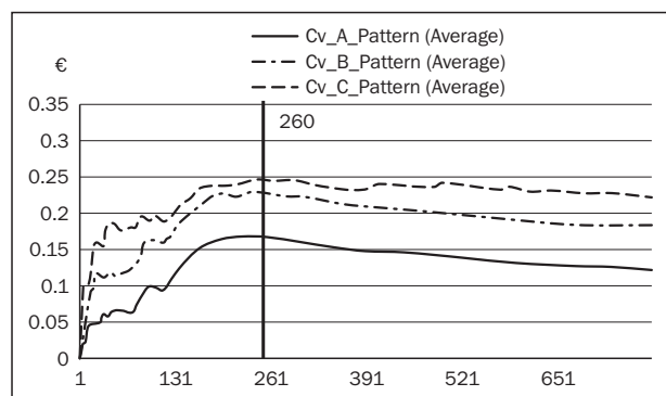
Figure 6 - Coefficient of Variation associated with the price patterns
