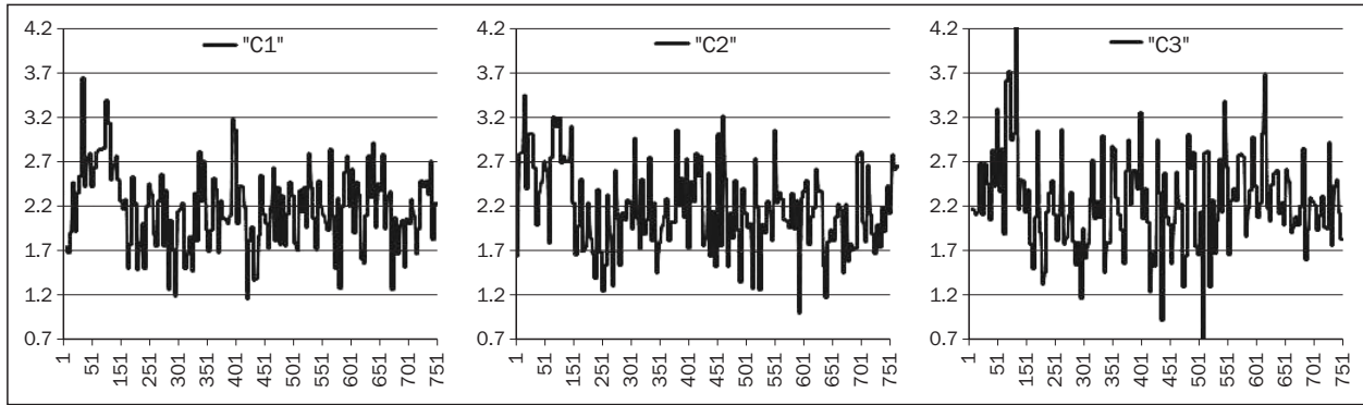
Figure 5 - Series disturbed by high variability
