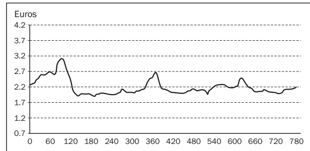
Figure 2 - Original price series
