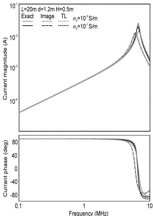
Fig. 6. Current at the feed point of a 20-m conductor at H = 0.5 m (thick layer d = 1.2 m)
