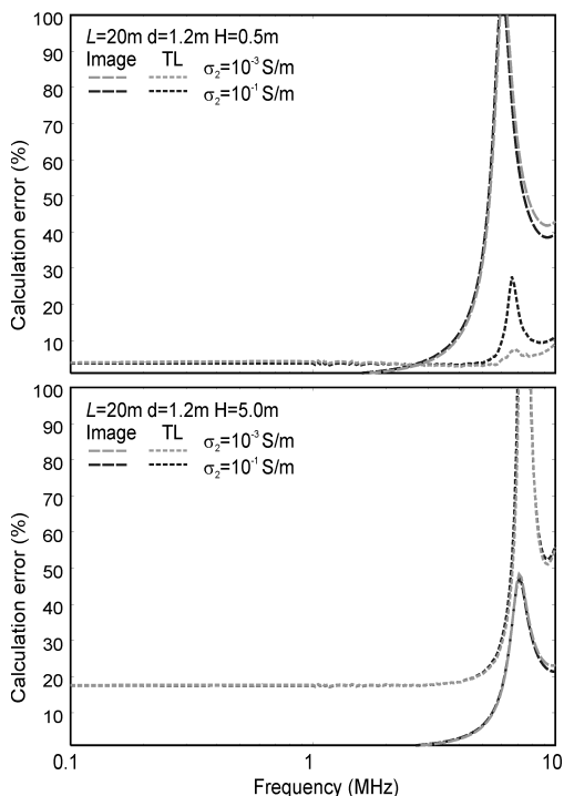
Fig. 9. Calculation error for 20-m conductor obtained by using Image and TL models for d = 1.2\text{m}
