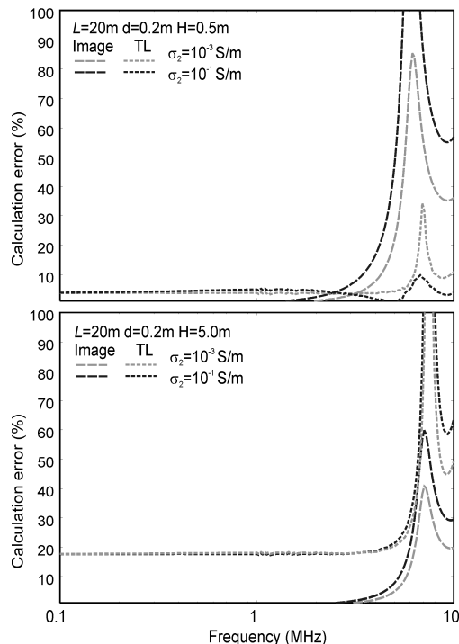
Fig. 8. Calculation error for 20-m conductor obtained by using Image and TL models for d = 0.2 m
