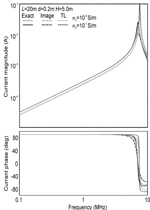
Fig. 5. Current at the feed point of a 20-m conductor at H = 5.0 m (thin layer d = 0.2 m)
