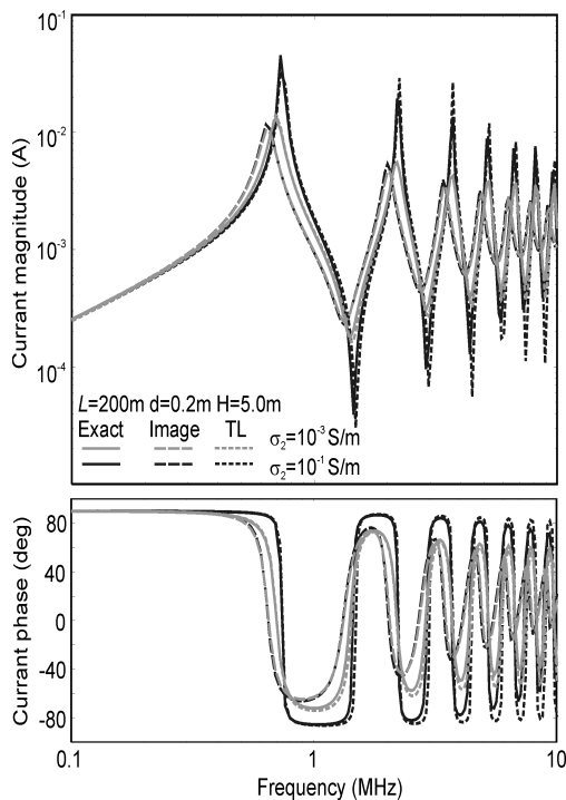
Fig. 12. Current at the feed point of a 200-m conductor at H = 5.0 m for d = 0.2 m
