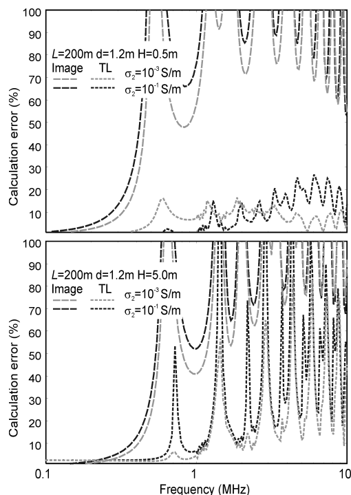
Fig. 16. Calculation error for 200-m conductor obtained by using Image and TL models for d = 1.2 m
