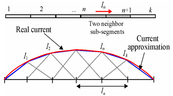
Fig. 2. Approximation of the current with roof-top basis functions over two neighbor segments
