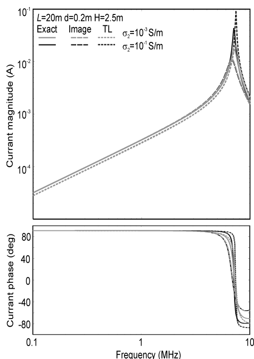
Fig. 4. Current at the feed point of a 20-m conductor at H = 2.5 m (thin layer d = 0.2 m)
