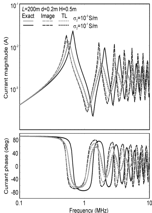
Fig. 10. Current at the feed point of a 200-m conductor at H = 0.5\text{m} for d = 0.2\text{m}
