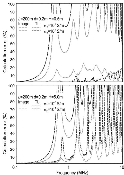
Fig. 15. Calculation error for 200-m conductor obtained by using Image and TL models for d = 0.2 m
