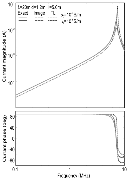
Fig. 7. Current at the feed point of a 20-m conductor at H = 5.0 m (thick layer d = 1.2 m)
