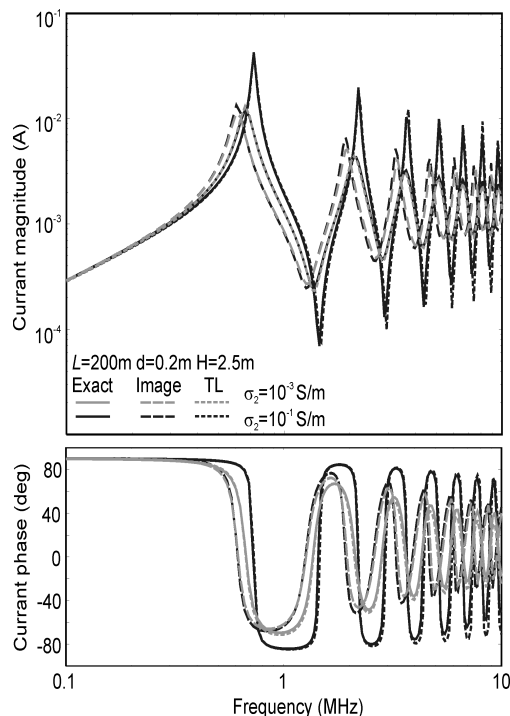
Fig. 11. Current at the feed point of a 200-m conductor at H = 2.5\text{m} for d = 0.2\text{m}
