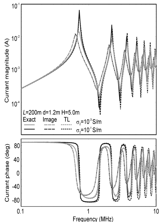
Fig. 14. Current at the feed point of a 200-m conductor at H = 5.0 m for d = 1.2 m
