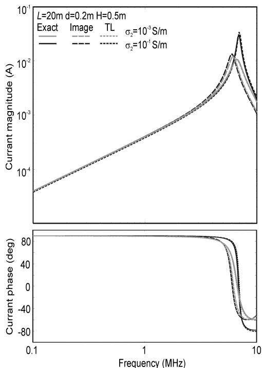
Fig. 3. Current at the feed point of a 20-m conductor at H = 0.5 m (thin layer d = 0.2 m)
