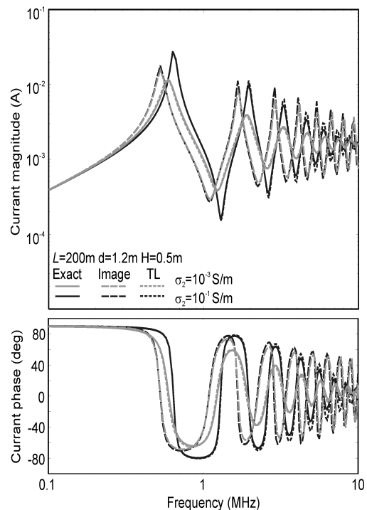
Fig. 13. Current at the feed point of a 200-m conductor at H = 0.5 m for d = 1.2 m
