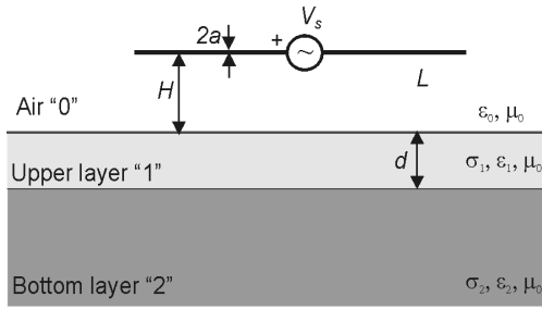
Fig. 1. A center fed horizontal wire conductor above two-layer soil
