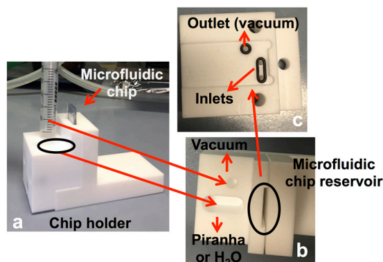
Figure 3. Pictures of the Teflon holder for Piranha activation of the channel interior: (a) chip holder overview, and top view of (b) bowl for inserting piranha or water, vacuum connection and reservoir for inserting the microfluidic chip and (c) chip holder reservoir for positioning chip inlets and outlet, respectively.
