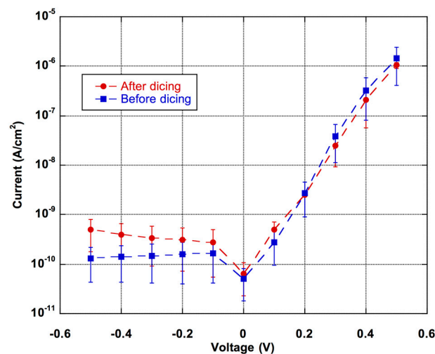
Figure 4. Current voltage characteristics of the a-Si:H photodiodes before (blue squares) and after (red circles) the dicing process. Symbols and bars refer, respectively, to the averaged values and to the standard deviations measured over five photodiodes.
