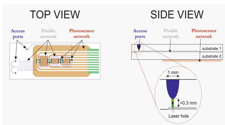
Figure 1. Schematic views of the design of the all-glass chip with integrated photosensors.
