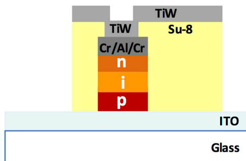
Figure 2. Cross section of the a-Si:H photosensor. Light is impinging through the glass substrate and the ITO (Indium Tin Oxide) bottom transparent electrode, before being absorbed by the p-i-n structure.
