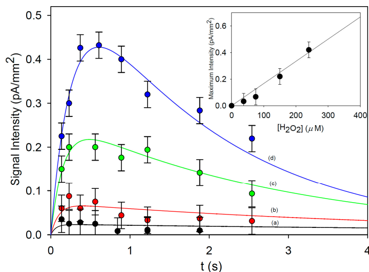
Figure 7. Signal intensity generated by the chemiluminescent decay of 2^* versus residence time in the chip ( [\text{I}] = 1.0 \text{ mM} , [\text{4-IOP}] = 0.10 \text{ mM} , T = 25 \text{ }^\circ\text{C} ). The measurements were carried out at four different \text{H}_2\text{O}_2 concentrations: 37.5 \text{ } \mu\text{M} (a), 75 \text{ } \mu\text{M} (b), 150 \text{ } \mu\text{M} (c), 240 \text{ } \mu\text{M} (d). Data points are experimental, and the solid line is the plot of Equation (1) with best fit k_2 = (2.5 \pm 0.3) \times 10^3 \text{ M}^{-1} \text{ s}^{-1} , k_c = 9.0 \pm 3.2 \text{ s}^{-1} . Inset: plot of the maximum signal intensity versus the initial concentration of \text{H}_2\text{O}_2 .
