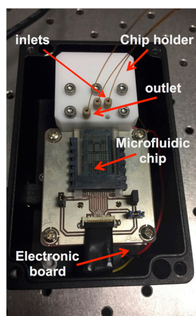
Figure 6. Picture of a horseradish peroxidase (HRP) functionalized chip connected to the electronic board for \text{H}_2\text{O}_2 detection.
