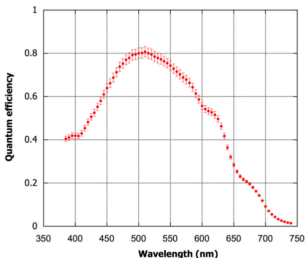
Figure 5. Spectral response of the photodiodes. Symbols and bars refer, respectively, to the averaged values and to the standard deviations measured over 5 photodiodes.
