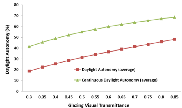
Figure 8: The relationship between glazing visual transmittance and average daylight autonomy (small glazing area).
