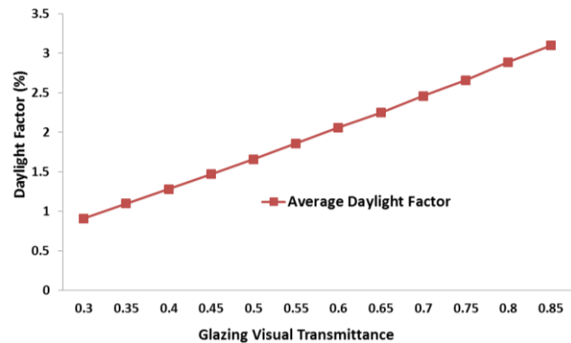
Figure 7: The relationship between glazing visual transmittance and average daylight factor (small glazing area).
