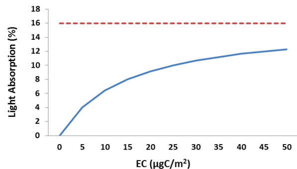
Figure 2: The impact of particulate elemental carbon amounts of glazing surface on the light absorption.
