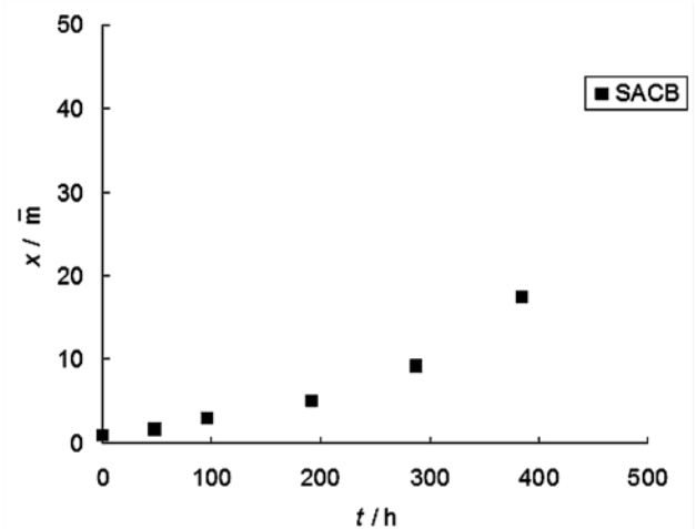
Figure 5 Thickness of the Cu_6Sn_5 layer versus ageing time for solder system SAC1.0B
