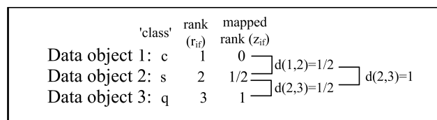
Fig. 4. Example: data object described with ordinal variable
