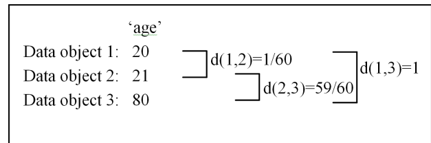
Fig. 3. Example: data object described with interval-scaled variable
