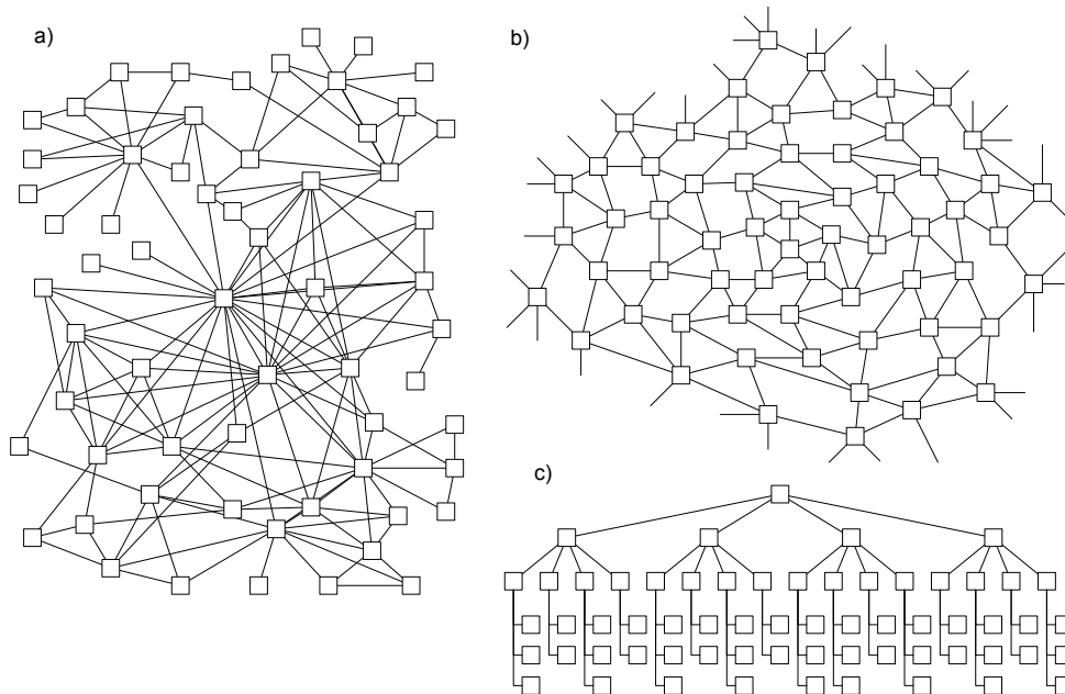
Figure 7. Three networks of different structural types with similar general properties: a) network with exponentially distributed degrees of nodes, b) network with uniformly distributed degrees of nodes, c) strictly hierarchical network.
