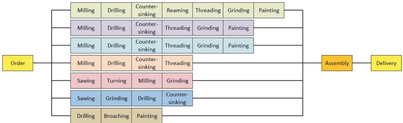
Figure 9 Main production process
