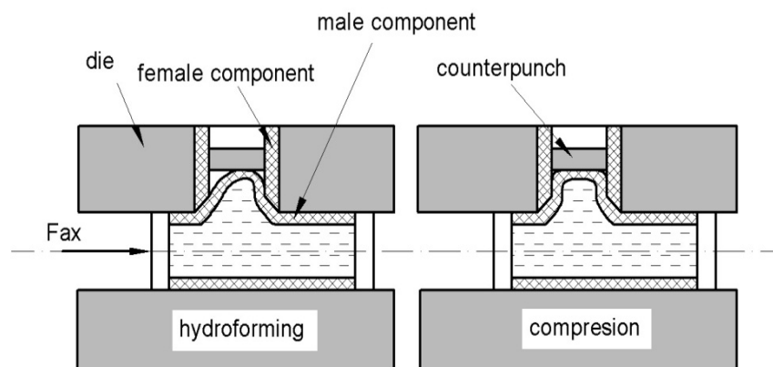
Figure 2. Angular joining by hydroforming [2]
