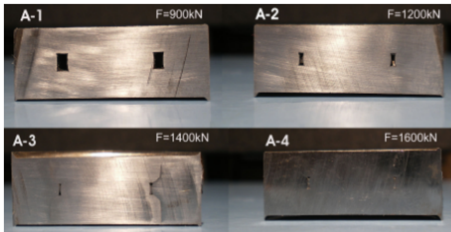
Figure 7. Cross section of cut bimetallic component
