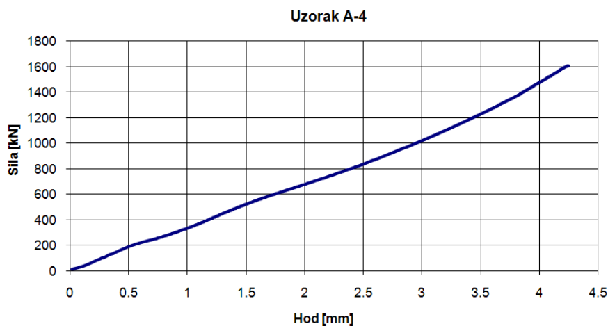
Figure 9. Load – stroke characteristic for the model A-4
