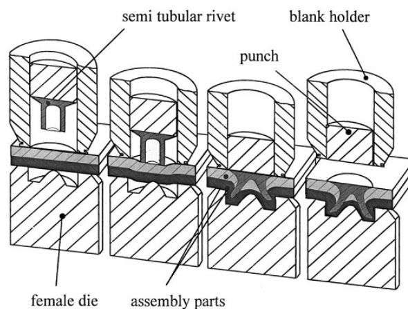
Figure 1. Self-piercing riveting technique [1]
