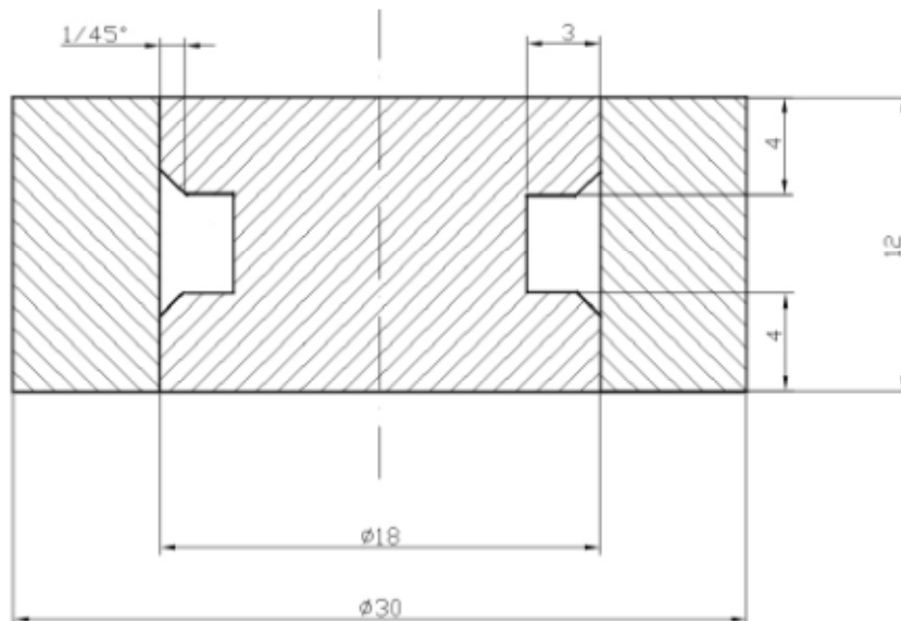
Figure 5. Dimensions of bimetallic components
