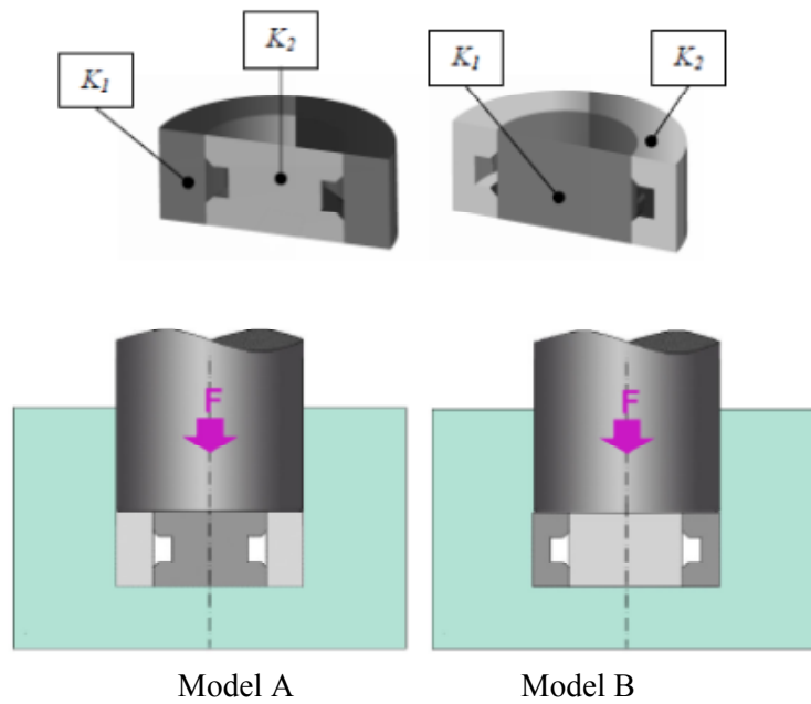
Figure 4. Two models of bimetallic joining
