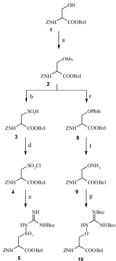
a) CH 3 SO 2 Cl/DIPEA/DMF; b) Na 2 SO 3 /H 2 O (or MW irradiation); c) N -Hydroxyphthalimide/NaH/DMF (or MW irradiation); d) SO 2 Cl/CH 2 Cl 2 ; e) mono-Boc-Guanidine/Et 3 N/DMF; f) N 2 H 4 ·H 2 O/EtOH; g) Boc 2 -pyrazole/CH 3 CN/DIPEA
