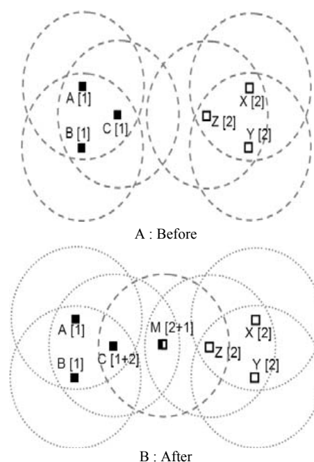
Figure 3. Sleep Schedule before and after node M join the network
