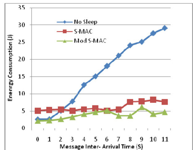
Figure 5. Energy Consumption
