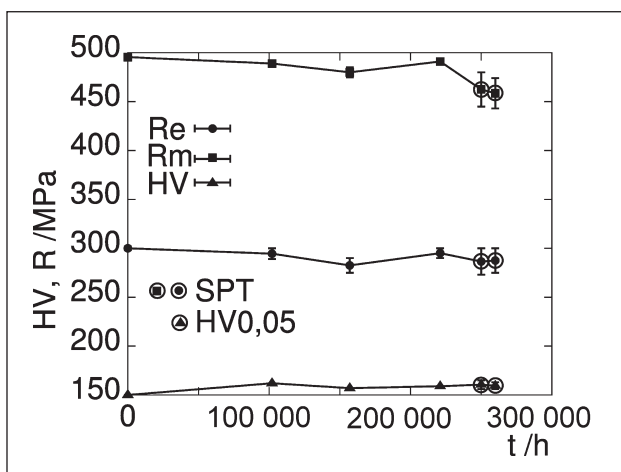
Figure 1 Influence of service life t on yield point R e strength R m and hardness HV. Service conditions 530 °C and stress level 46,5 MPa
