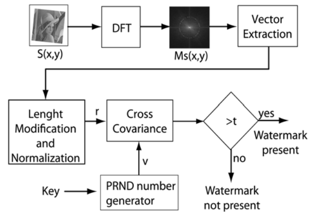
Figure 4 Block diagram of the decoder Slika 4. Blok dijagram dekodera
