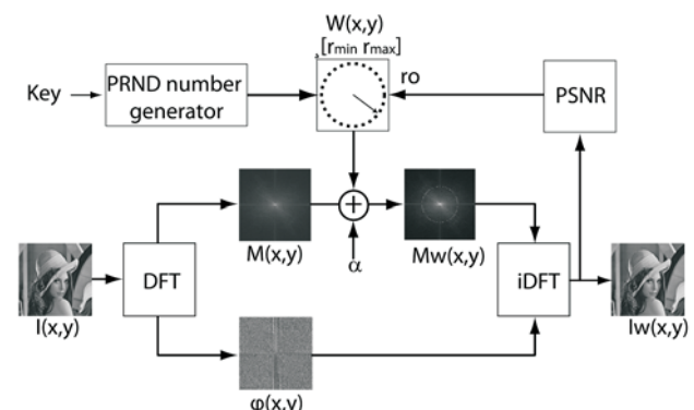
Figure 2 Block diagram of the encoder Slika 2. Blok dijagram enkodera
