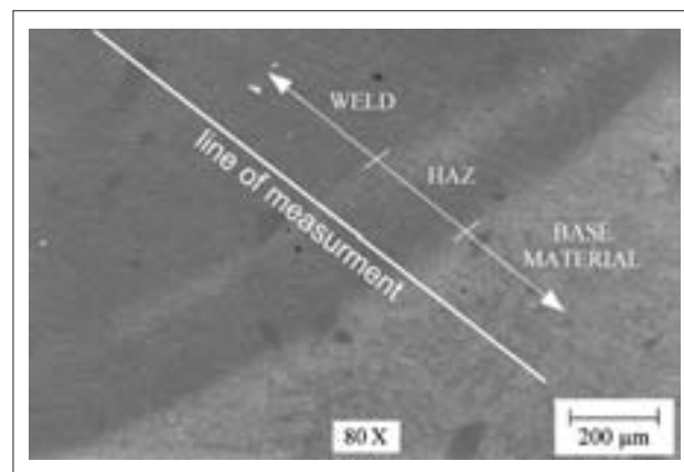
Figure 6 Heat-affected zone between the surface weld made of copper alloy and AlCu
