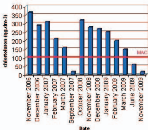
Figure 7. Fluctuation of chlortoluron concentration in drainage water for drainpipe spacing of 15 m
