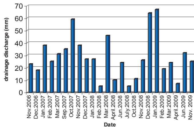
Figure 5. Fluctuation of drainage discharge (mm) for drainpipe spacing of 15 m
