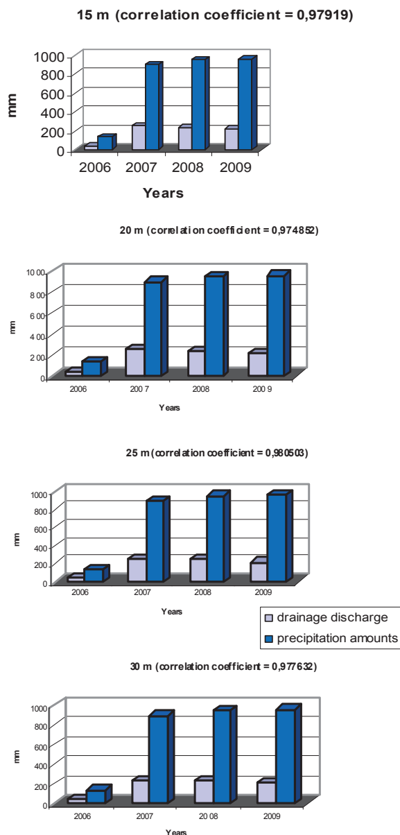
Figure 4. Correlation coefficients between precipitation (mm) and drainage discharge (mm) for drainpipe spacing: 15, 20, 25 and 30 m
