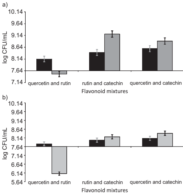
Fig. 3. Number of viable cells of Listeria monocytogenes in BHI medium supplemented with: a) 100 or b) 200 mg/L of different flavonoid compound mixtures. (■) Theoretical values, (▒) experimental values. Each point represents the average value of three determinations
