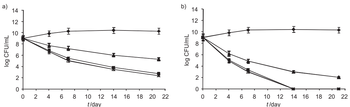
Fig. 1. Survey of L. monocytogenes in meat supplemented with phenolic compound mixtures at 4^{\circ}\text{C} : a) 100 and b) 200 mg/L. (♦) Control, (▲) gallic and protocatechuic acids, (■) gallic and caffeic acids and (x) rutin and quercetin. Each point represents the average value of three determinations
