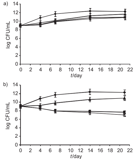
Fig. 4. Survey of L. monocytogenes in meat supplemented with phenolic compound mixtures at 20 °C: a) 100 and b) 200 mg/L. (◆) Control, (▲) gallic and protocatechuic acids, (■) gallic and caffeic acids and (x) rutin and quercetin. Each point represents the average value of three determinations
