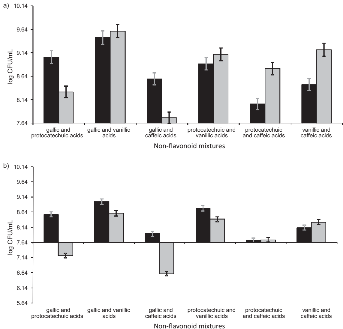
Fig. 2. Number of viable cells of Listeria monocytogenes in BHI medium supplemented with: a) 100 or b) 200 mg/L of different non-flavonoid compound mixtures. (■) Theoretical values, (▒) experimental values. Each point represents the average value of three determinations
