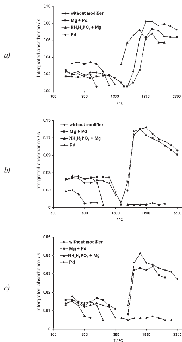
Figure 1 Pyrolysis and atomisation curves in the absence and in the presence of different modifiers for: a) standard solution ( 20 \mu\text{g L}^{-1} ); b) red wine sample (dilution 1:1); c) white wine sample (dilution 1:1)
