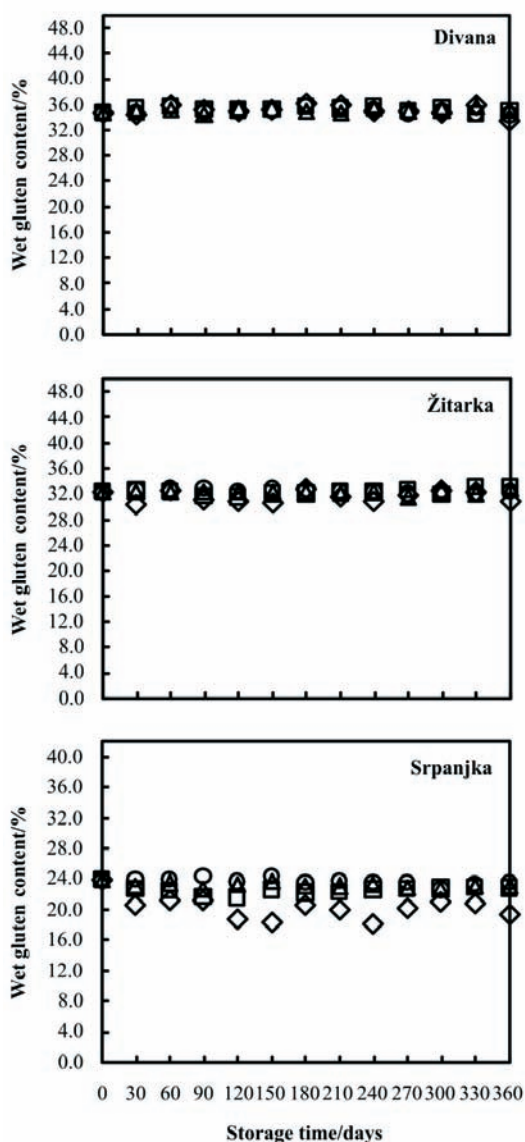
Figure 4. Wet gluten content of three wheat varieties during storage at different conditions. Storage conditions: 40°C, RH = 45% (◇); 25°C, RH = 45% (□); 4°C, RH = 45% (△); 2-25°C, RH = 40-74% (○)
