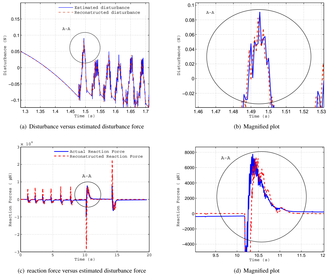
Fig. 6. Disturbance and reaction forces versus estimated disturbance and reaction forces
