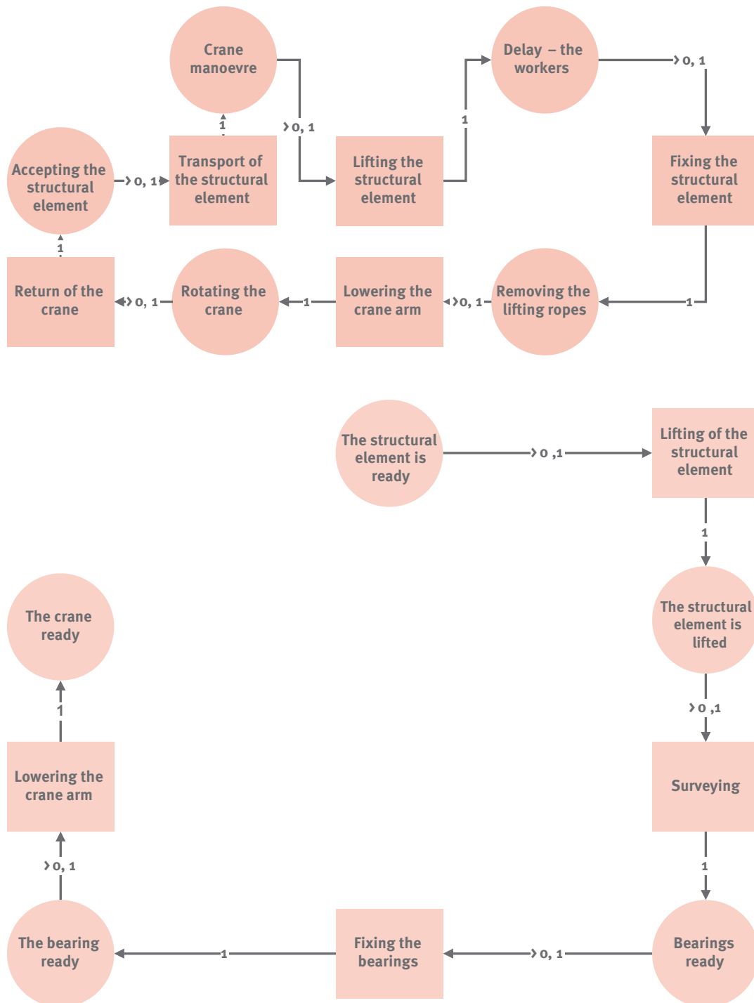
Figure 1. The Stroboscope model for jobsite transportation and manual installation of a single heavy structural element
