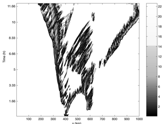
Figure 5: Hovmöller diagram of rainrate ( \text{mm hr}^{-1} ) for the SM7 case.
