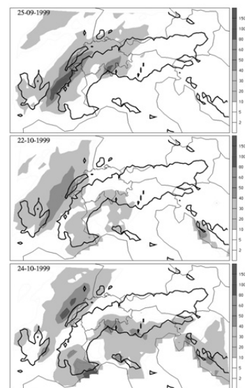
Figure 1: The 24 h accumulated precipitation starting at 06 UTC on the day given in the upper left of each panel.
