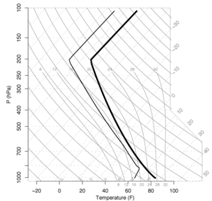
Figure 2: Sounding used to initialize simulations (temperature - black, dew point temperature - red) from Weisman and Klemp 1982).
