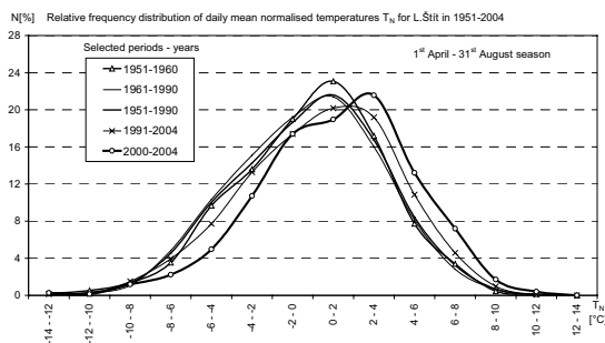
Figure 5. Left - frequency distribution N[\%] of temperature daily means T[^\circ\text{C}] at the station LŠ in 1951-2004; Right – frequency distribution N[\%] of humidity daily means U[\%] at the station LŠ in 1951-2004 (deviations from the 1951-2000 averages for each day in the April-August season).
