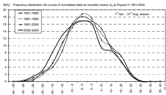
Figure 6. Left - frequency distribution N[\%] of humidity daily means U[\%] at the station HU in 1951-2004 (deviations from the 1951-2000 averages for each day in the April-August season); Right – frequency distribution N[\%] of humidity daily means U[\%] at the station PO in 1951-2004 (deviations from the 1951-2000 averages for each day in the April-August season).
