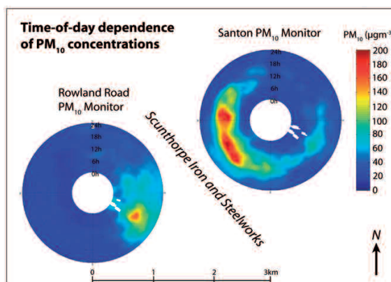
Figure 2. Time-of-day dependence of PM 10 concentrations at Rowland Road and Santon monitor.
