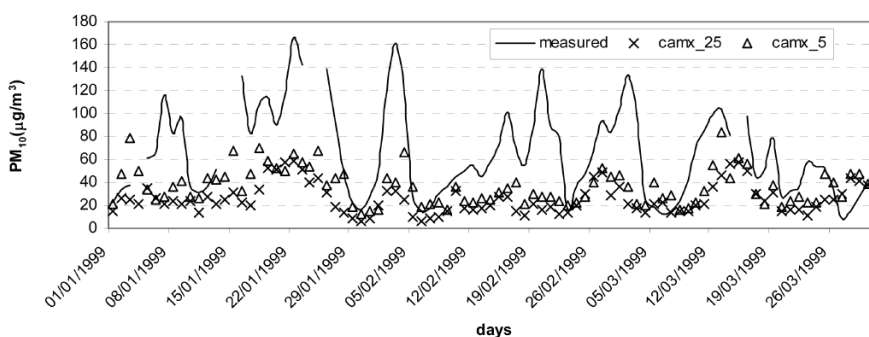
Figure 2. Mean daily PM 10 concentration at urban site 4 for the first period.
