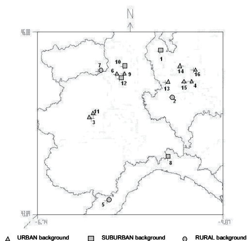
Figure 1. Simulation domain and monitoring sites
