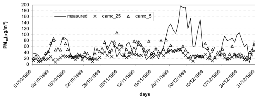
Figure 3. Mean daily PM 10 concentration at urban site 4 for the second period.
