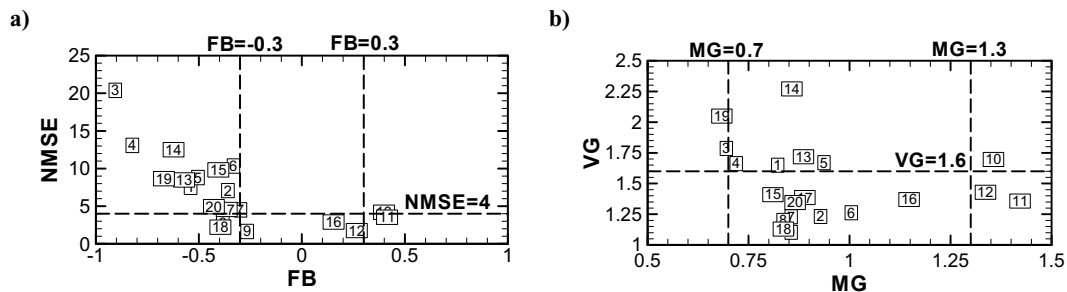
Figure 4. Metrics for the concentrations C^* of the -45 degree case. a) NMSE vs. FB , b) VG vs. MG .
