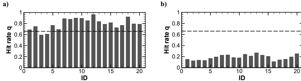
Figure 2. Hit rate for mean velocity components at the towers for the -45 degree case. a) U/U_{ref} b) W/U_{ref} .
