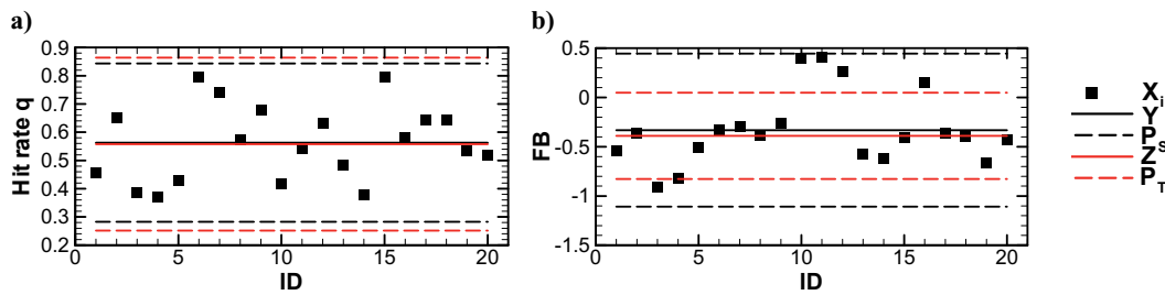
Figure 5. Running records of the metrics for the concentrations C^* of the -45 degree case. a) Hit rate q , b) FB .
