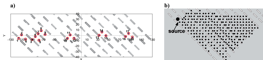
Figure 1. Measurement positions for the -45 degree case. a) towers for velocities, b) concentrations. Wind blows from the left.
