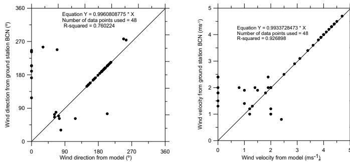
Figure 3a. Comparison for wind directions and wind speeds at BCN station.
