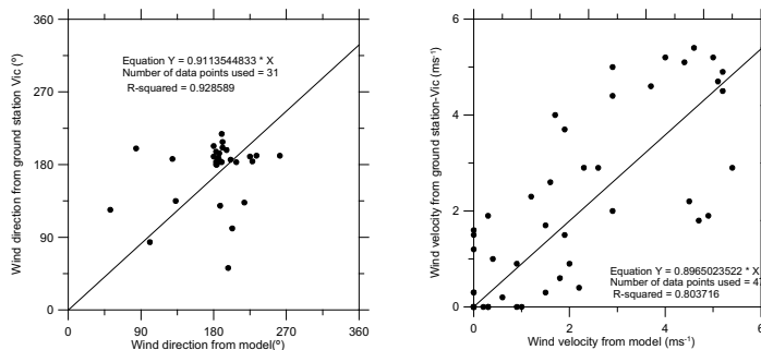
Figure 3b. Comparison for wind directions and wind speeds at Vic station.
