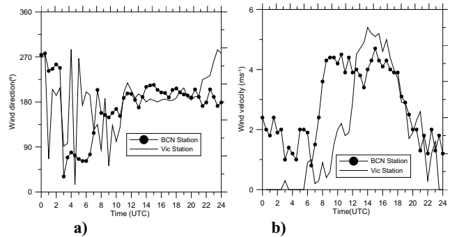
Figure 2. Temporal evolution of wind direction (a) and wind speed (b) at two stations: (BCN) located near the coast, and (Vic) located inland.
