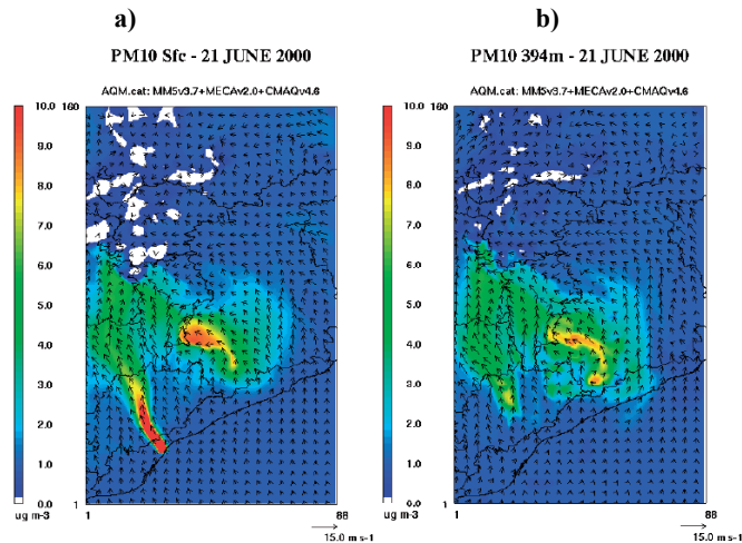
Figure 7. Horizontal cross section at 1400 UTC for the PM10 concentration in \mu\text{g m}^{-3} (colour scale) simulated by CMAQ model and horizontal wind velocity (vectors) simulated by the MM5 model: a) at 10 m above ground level and b) at 394 m above ground level.
