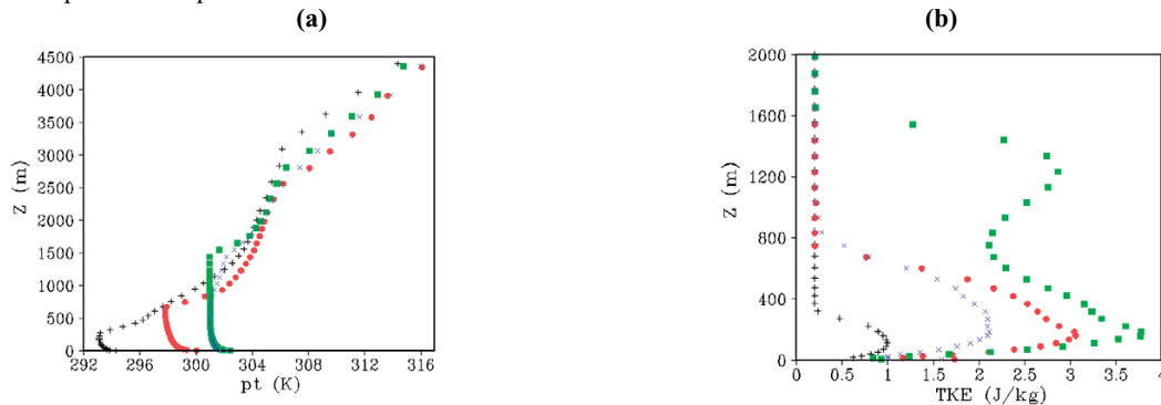
Figure 6. Vertical profiles for simulated potential temperature (a) and turbulent kinetic energy (b). At points: (1) in black at 0800UTC; point (2) in red at 1300 UTC; point (3) in green at 1120 UTC; and point 4 in blue at time 14 UTC.
