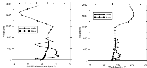
Figure 5. Comparison between vertical profiles of measured and modelled values for S-N wind components and wind direction.
