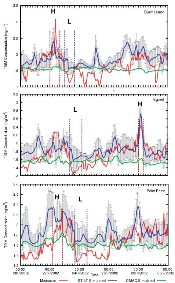
Figure 2. Comparison between observed and modeled TGM concentrations for 20 to 30 July.
