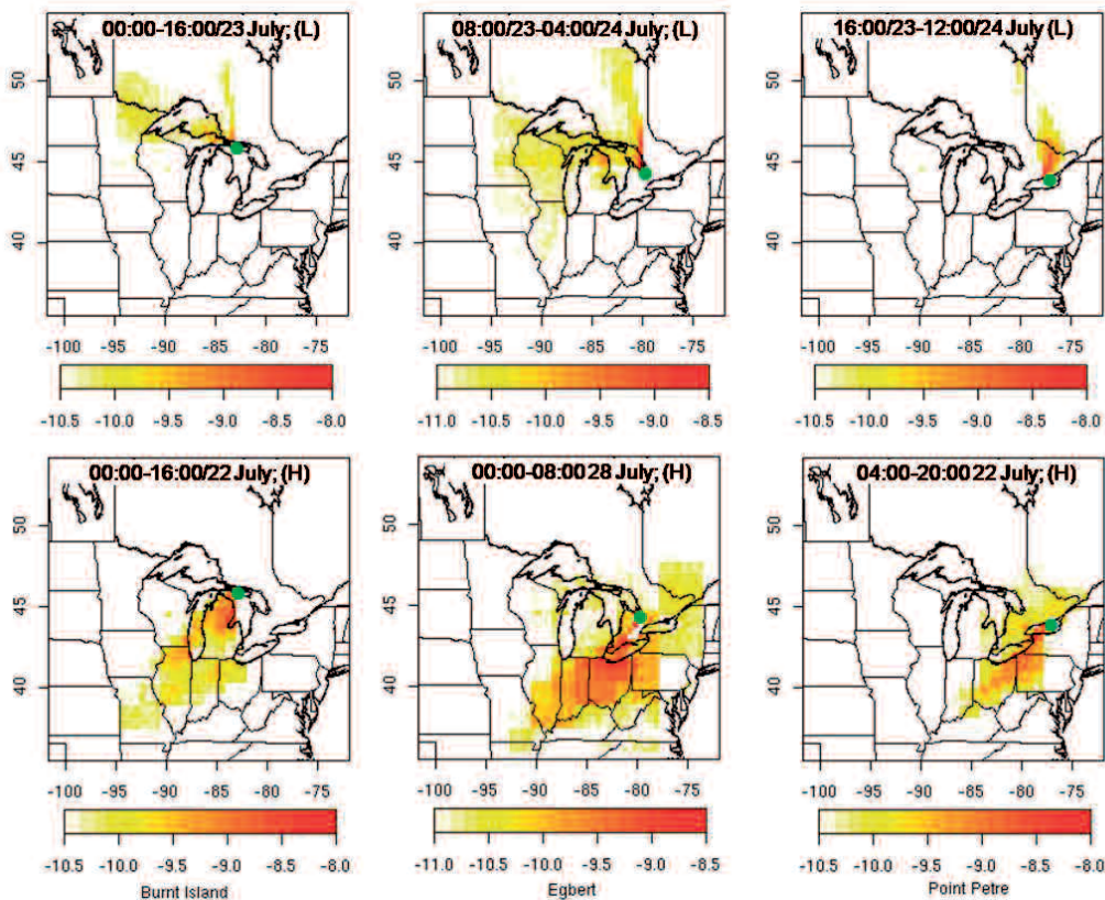
Figure 3. Source footprints for measured TGM episodes shown in Figure 2. The source footprint is the sum of the TGM content of all air parcels arriving during the indicated time period. The TGM content is the difference between the TGM emitted into and lost from the air parcel during the trajectory, as explained above.
