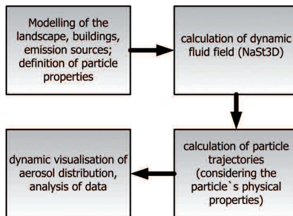
Figure 1. Flow chart of STAR3D
