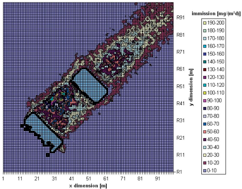
Figure 3. Immission of PM10 in simulation area.
