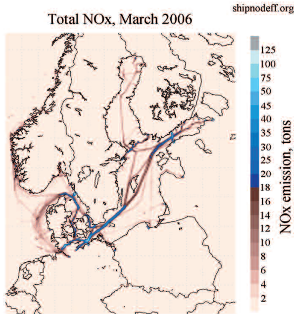
Figure 2. Total NO x release of ship traffic during March 2006.
