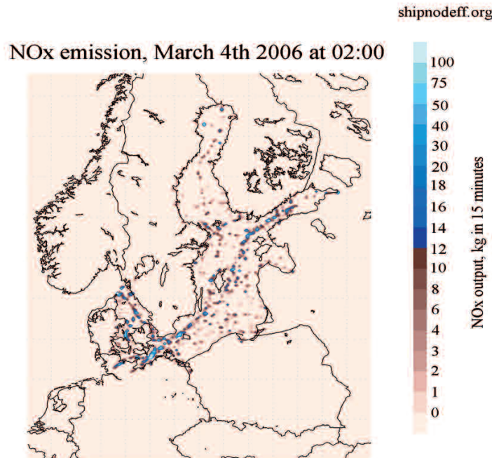
Figure 1. NO x emissions of ship traffic in the Baltic Sea area during one 15-minute period on March 4th 2006.
